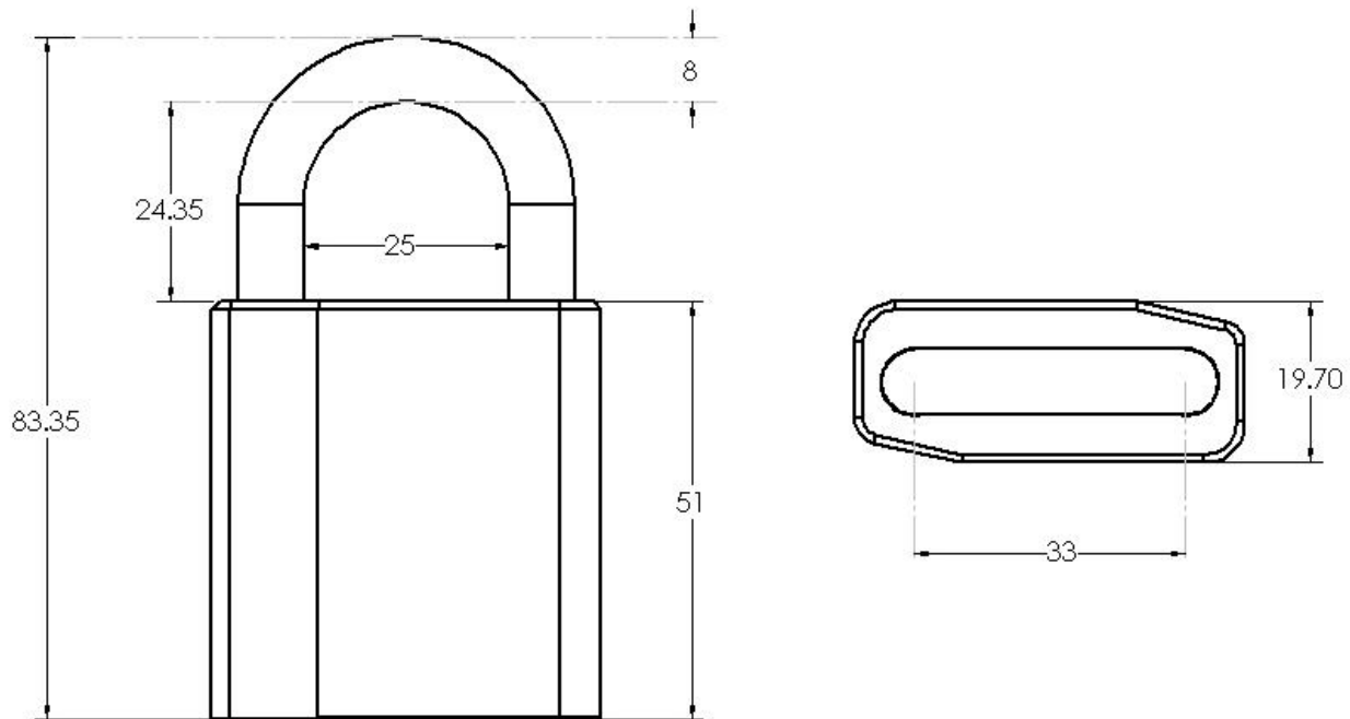
Figure 1: Padlock dimensions (mm)
